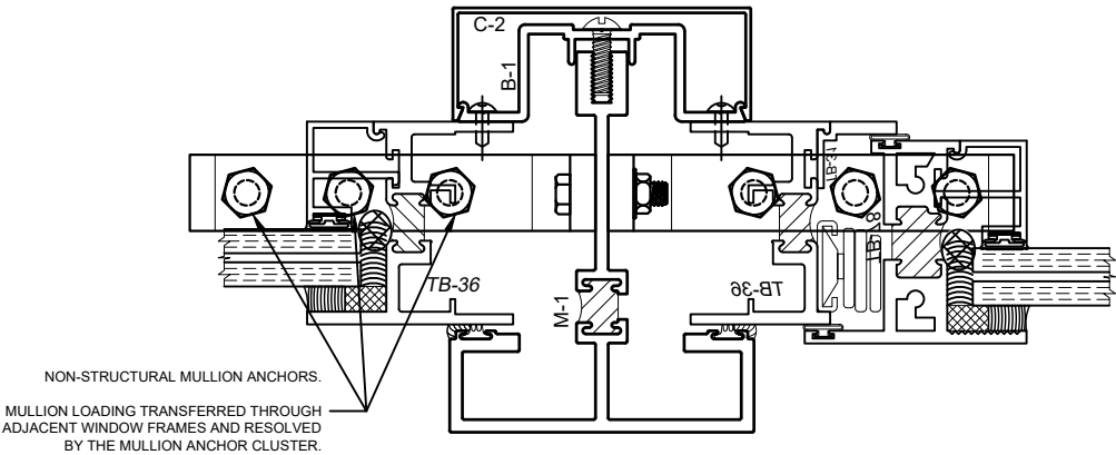
SECTION B: ANCH4 (HEAD SIMILAR) ATTACHMENTS AT MULLION
