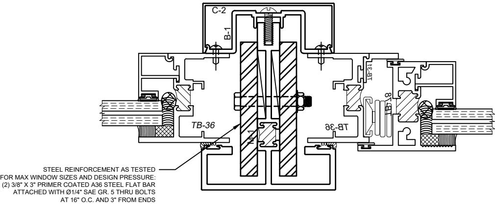
SECTION A: STEEL REINFORCEMENT
